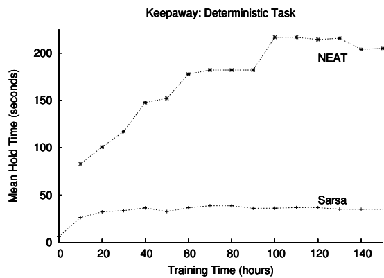
Figure 7: A comparison of the mean hold times of the policies discovered by NEAT and Sarsa in the deterministic version of the Keepaway task.
